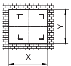
Dimensions of the internal climbing opening
